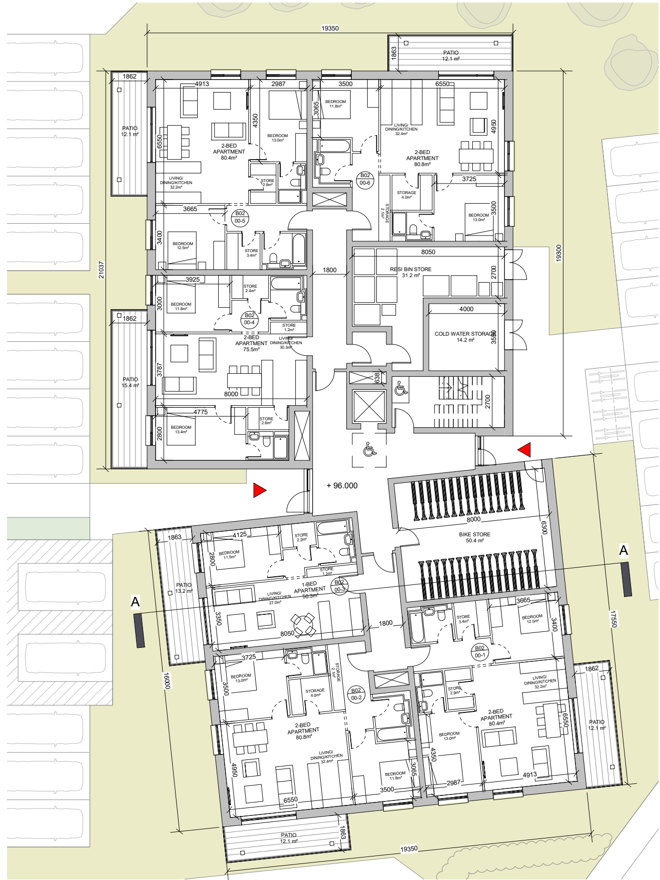
1 Block 02 - Level 00 1 : 200
